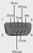
DB9M in RS232 Mode
